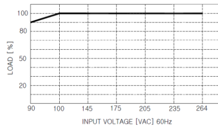
Load vs Input Voltage
