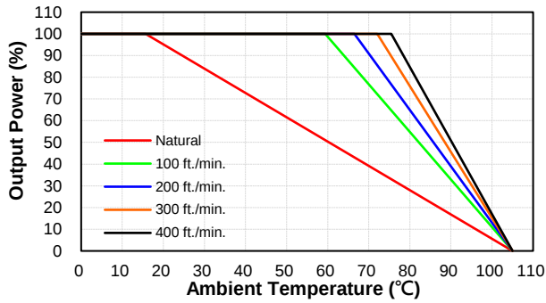
CQB150W8-36S24 Derating Curve with Heatsink QBT210 (Vin=3V)
